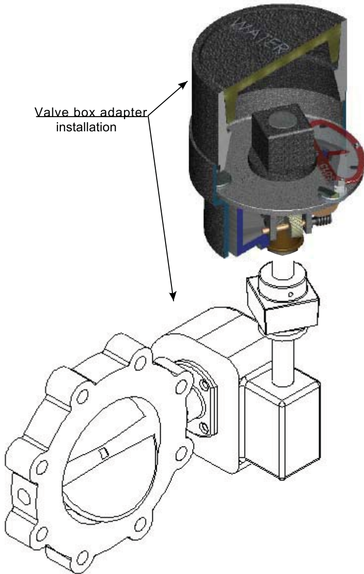
Typical Indico position indicator installation
